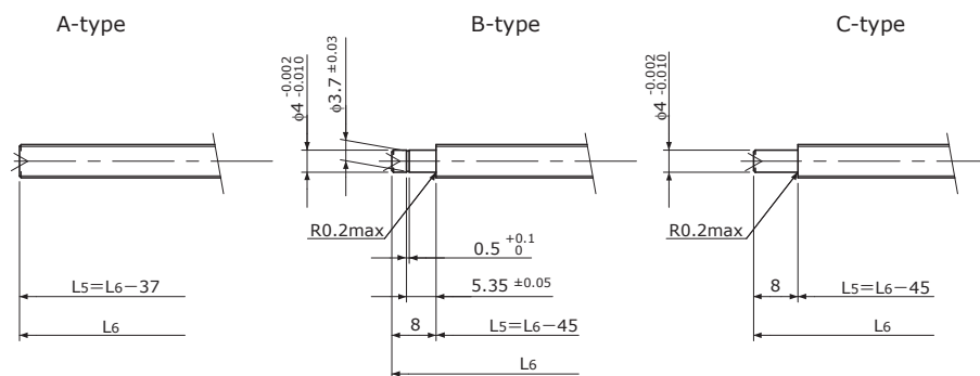
Supported-side end-journal profile 支撑侧轴端加工形状
