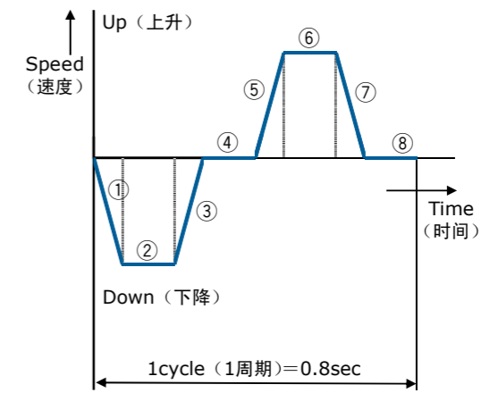
Operating pattern (运行周期线图)
