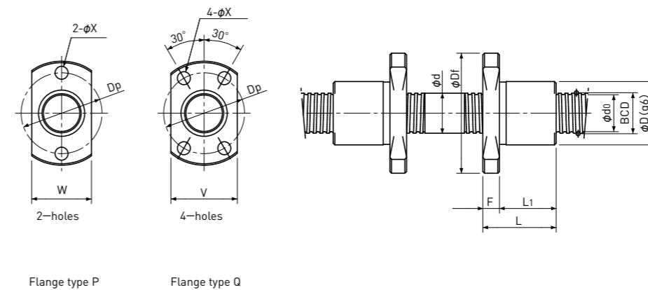
Type-2:Internal-deflector type
