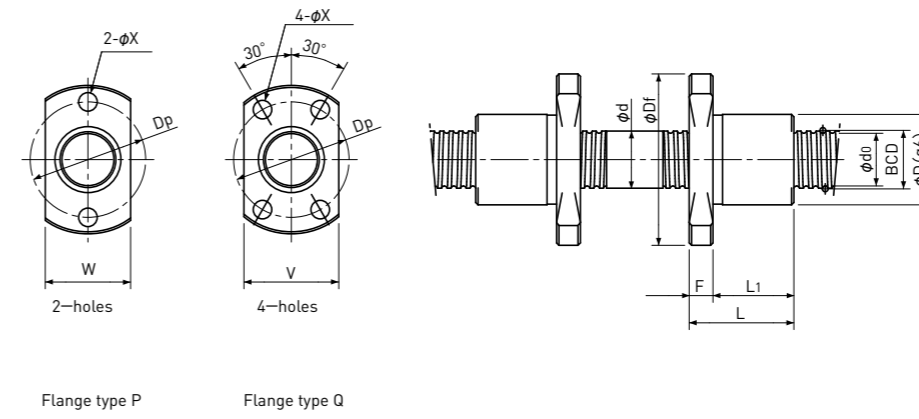
Type-2:Internal-deflector type
