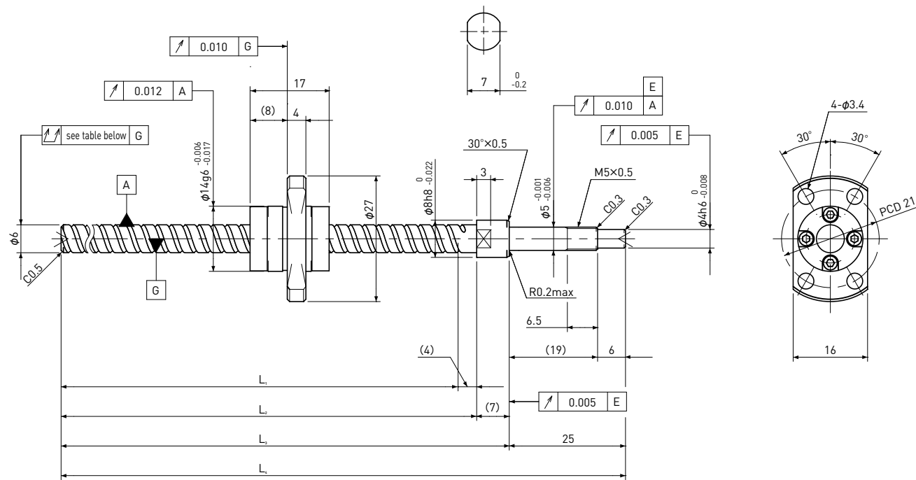
Supported-side end-journal profile
