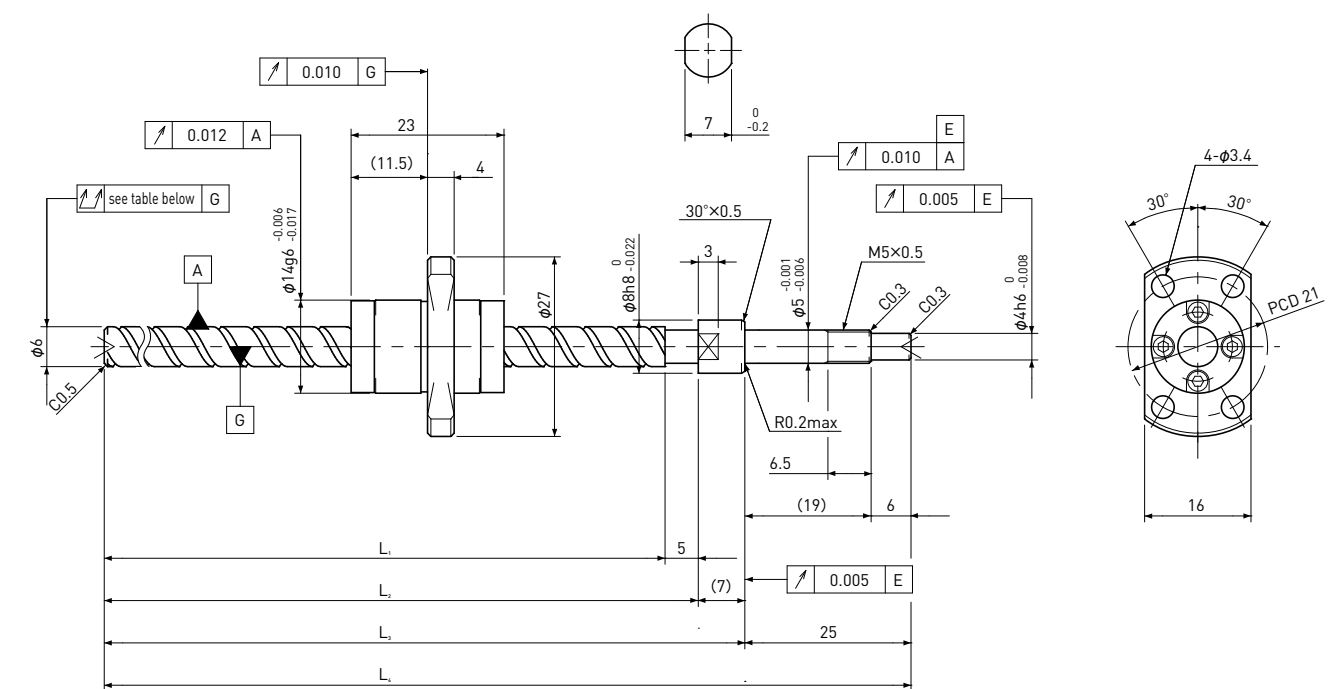
Supported-side end-journal profile
